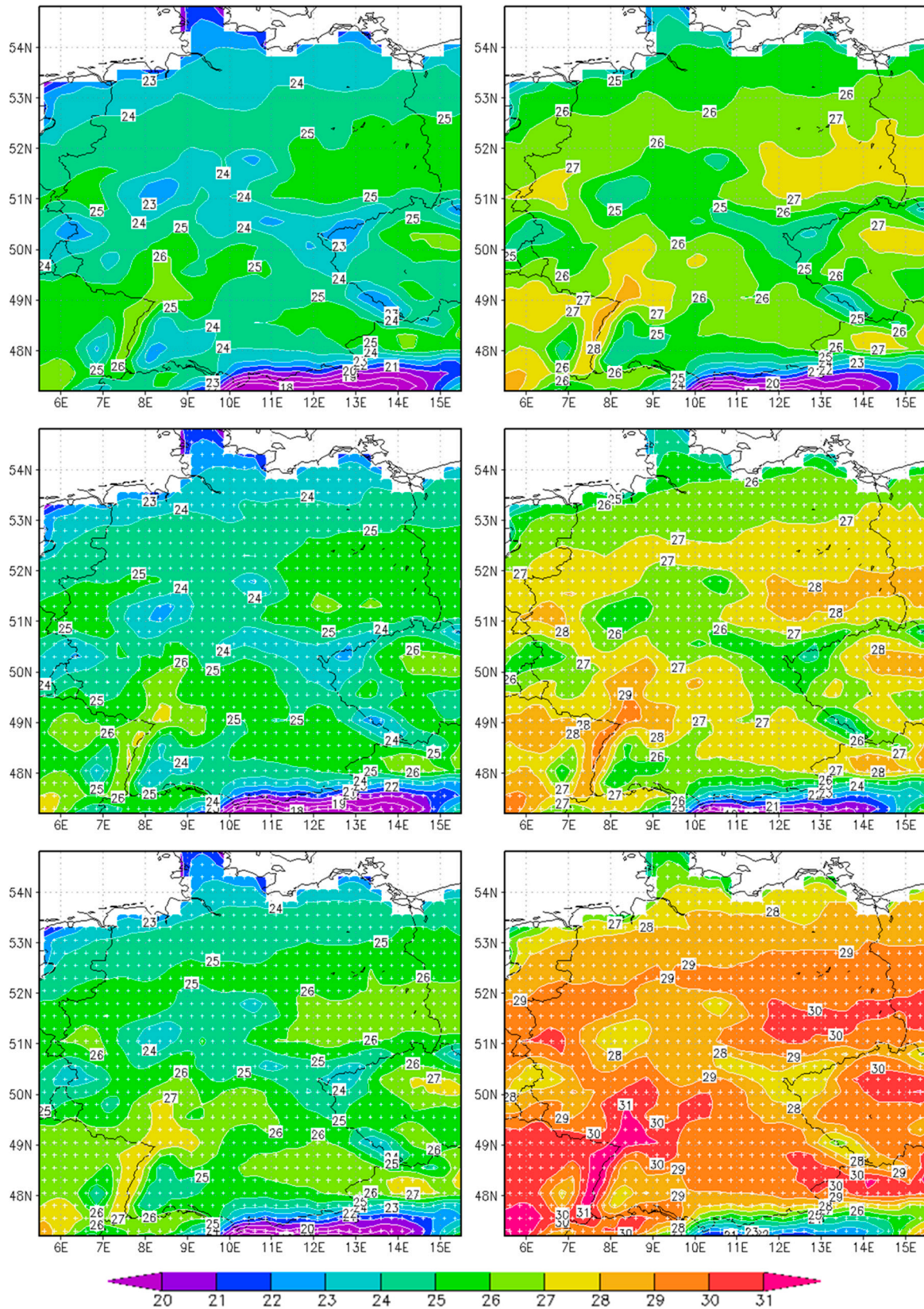
Figure 3. Projected ensemble mean of the average heat wave intensity ( left ) and amplitude ( right ) in degrees Celsius for 1971–2000 ( top ), 2021–2050 ( center ) and 2069–2098 ( bottom ). Grid points with significant changes ( \alpha < 0.05 ) between present and future climate are marked by white crosses.
